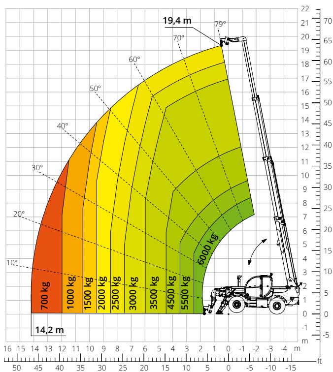
Load chart with HOOK, 6,000 kg ATT-05-001
