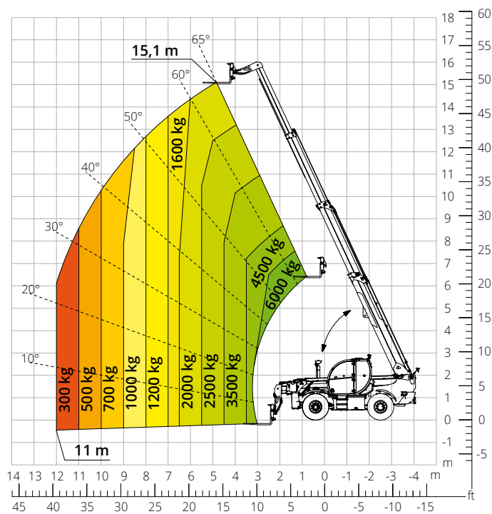
Load chart FRONT ATTACHMENT ON TYRES ATT-03-012
