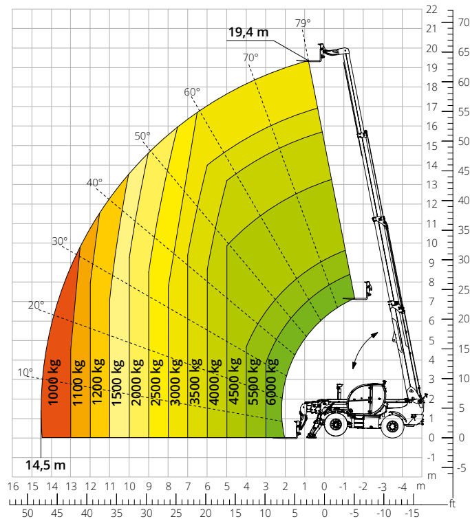
Load chart with FULLY EXTENDED STABILISERS (360°) ATT-03-012
