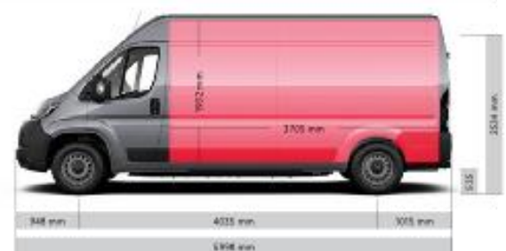
FURGON – L4H3 – 17 m 3
